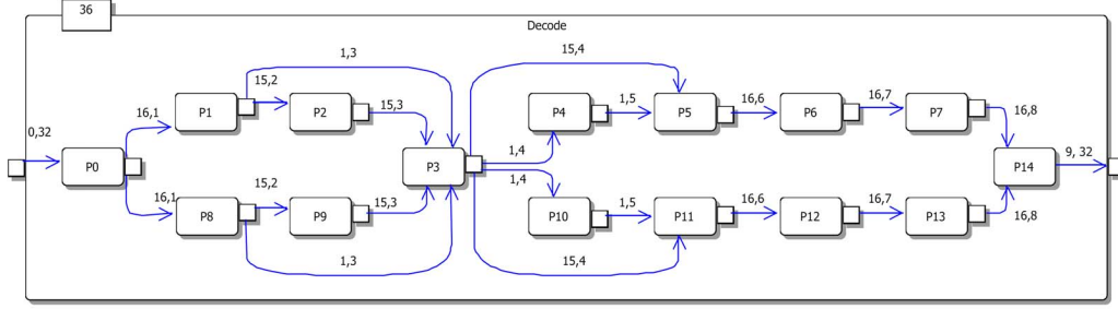
Figure 6. Partitioned application model of MP3 decoder.
