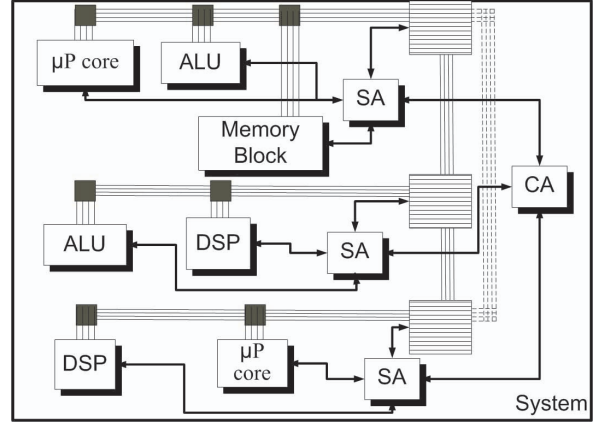
Figure 1. Segmented bus structure.
