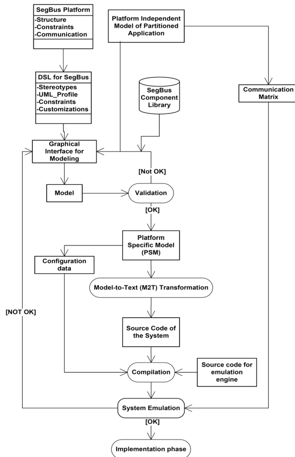
Figure 3. Design process of the SegBus platform using DSL and emulation.
