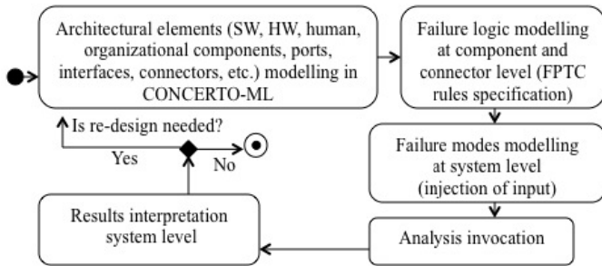
Fig. 1. Activity Diagram Related to CONCERTO-FLA
