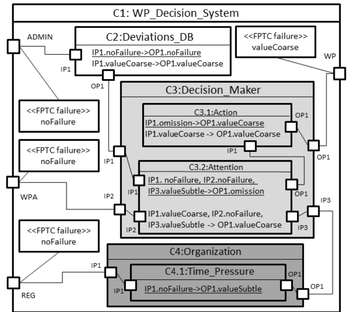
Fig. 3. Scenario 1: CONCERTO-FLA analysis results
