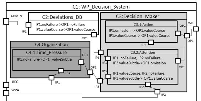
Fig. 2. CONCERTO-FLA architectural model
