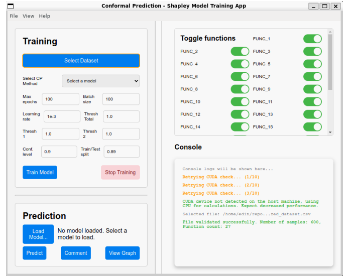
Fig. 6: Initial GUI screen - The left hand side is divided into Training and Prediction sections. The Training section uses user input for various general model training parameters, the Prediction section controls the loading of a trained model, annotations and graph window. The right hand side is divided into the Toggle section where tasks are toggled On/Off for prediction and the Console section where various information, warnings and errors are shown to the user.
