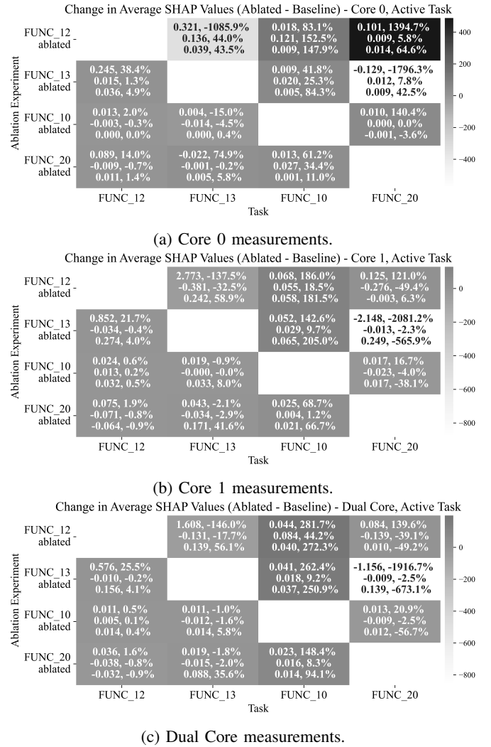
Fig. 11: Change in Shapley values of most significant tasks in ablated vs. baseline cases for the task's contribution when active. Values on the bottom represent the lower bound contribution, values in the middle are the prediction contribution, and values on top are the upper bound contribution.
