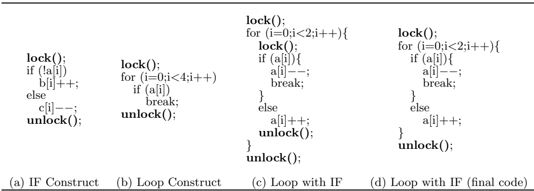
Figure 2: Non-analyzable codes with lock instructions.
