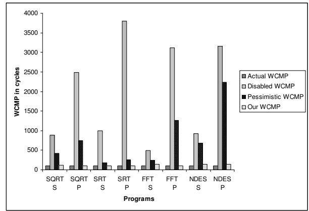
(b) Accuracy of our WCMP estimate.
