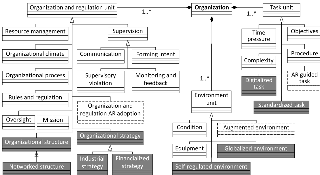
Fig. 4. Extended organization modeling elements [11].
