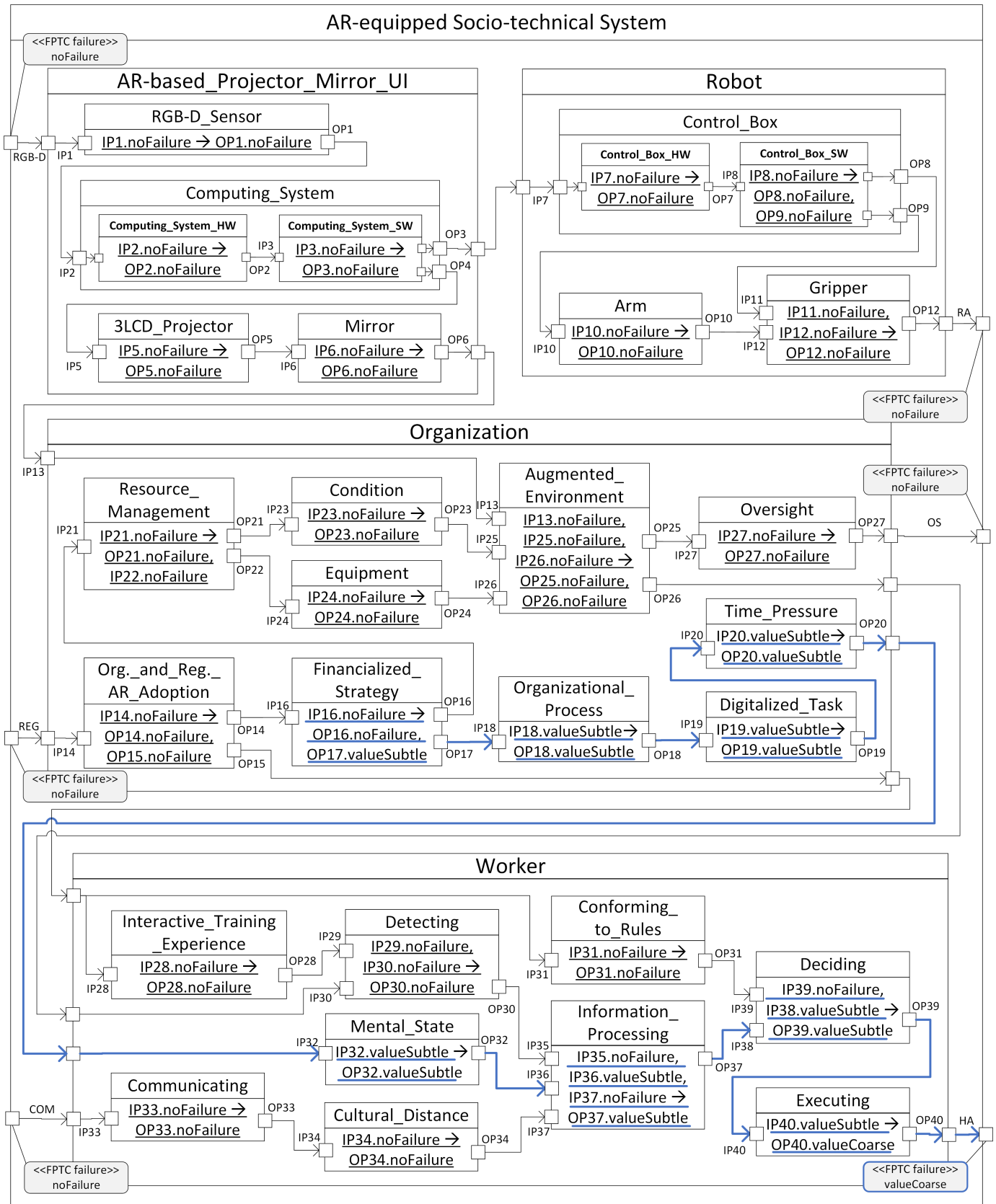
Fig. 11. Analyzing the AR-equipped socio-technical system (Scenario 1).
