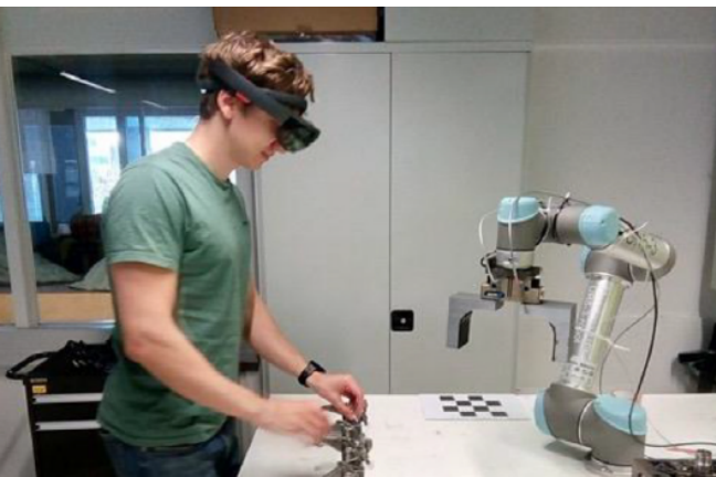
Fig. 8. Robot and Human using AR-based wearable HoloLens UI [35].
