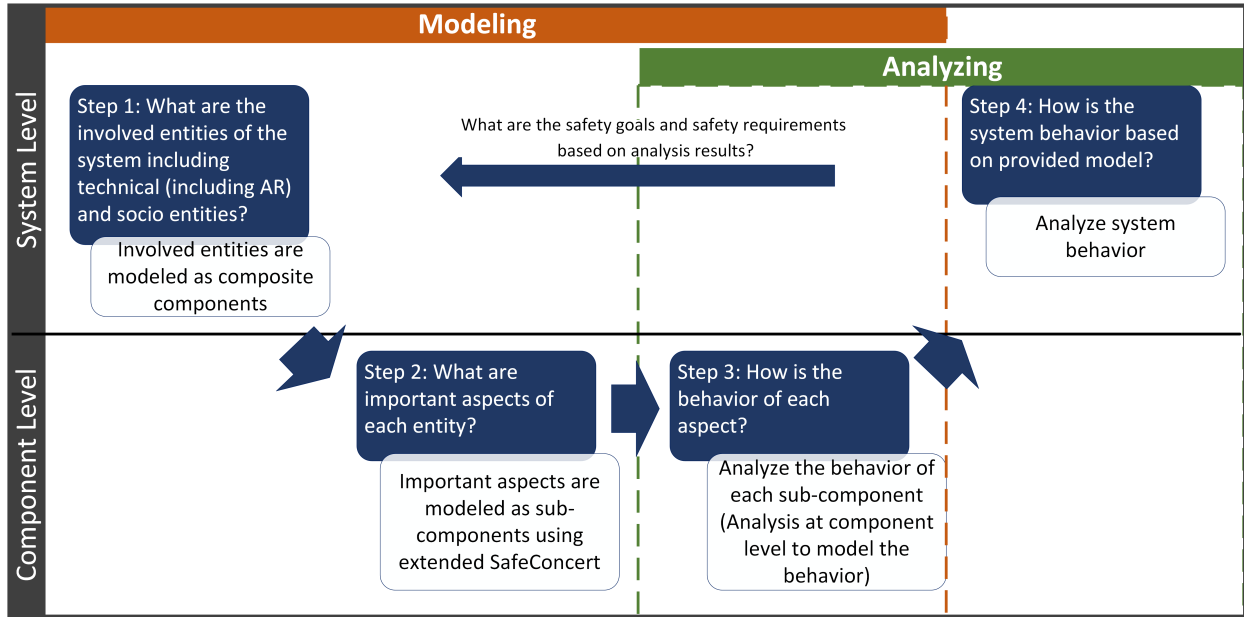
Fig. 2. Methodology of the FRAAR framework [10].
