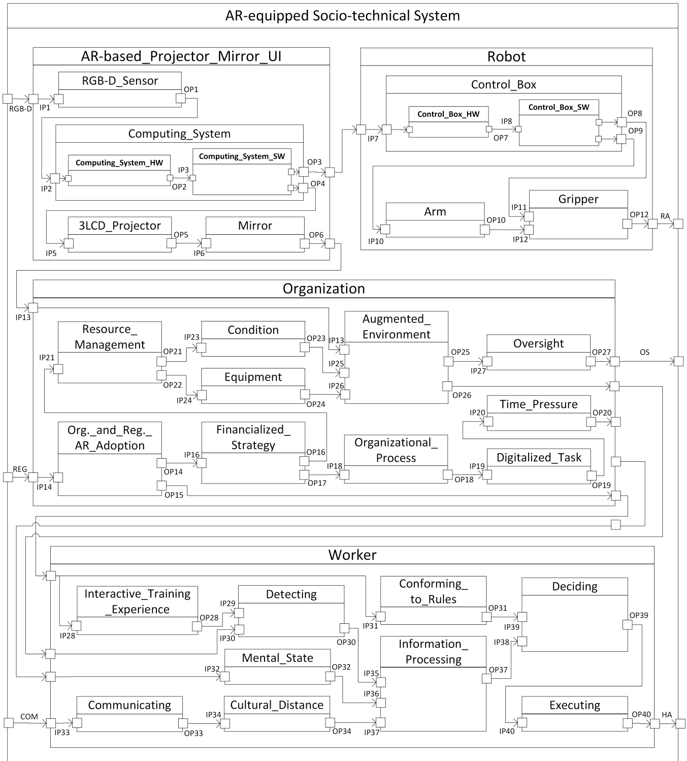
Fig. 10. Modeling of the AR-equipped socio-technical system
