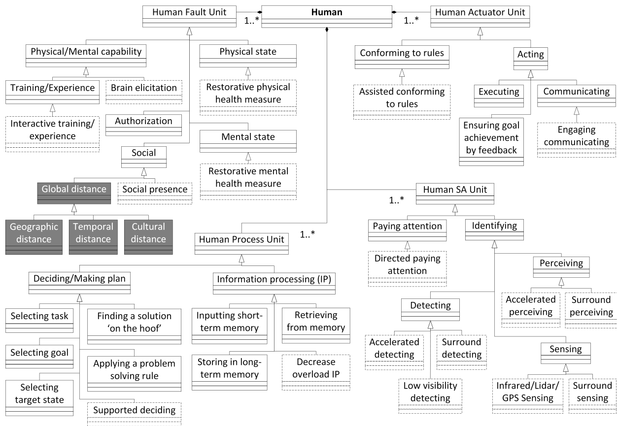
Fig. 3. Extended human modeling elements [11].
