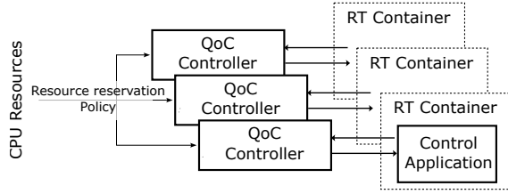
Fig. 3. Multiple controllers.
