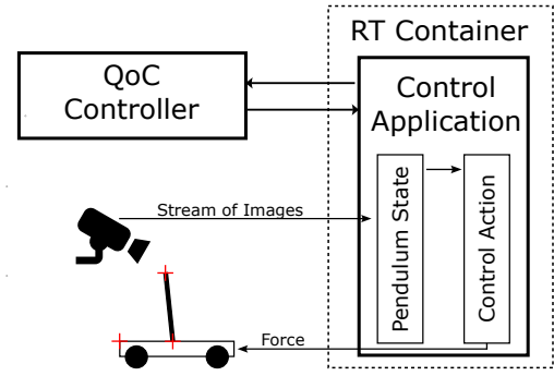
Fig. 4. Inverted pendulum experiment.
