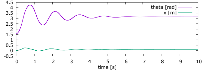
Fig. 5. Inverted pendulum use-case.
