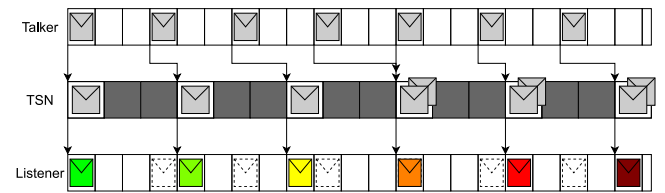
FIGURE 7. Positive legacy system clock drift behavior.
