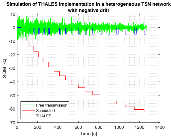
FIGURE 20. Simulation results of the implemented heterogeneous TSN network with negative drift.
