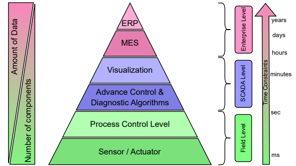
FIGURE 1. Automation Pyramid.
