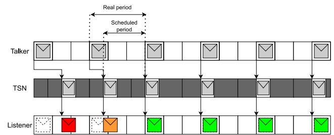
FIGURE 10. TALESS operating diagram.
