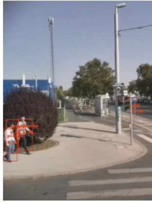
Fig. 10. Object detection [160].
