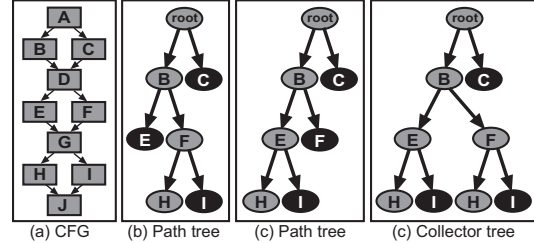
Figure 2. Example CFG and Path Trees
