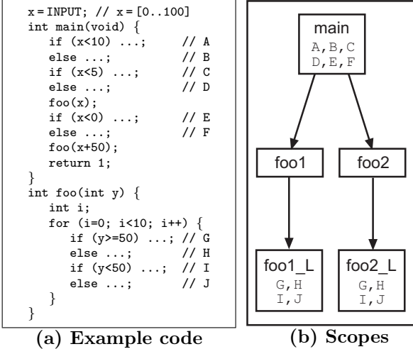
Figure 3. Code with several infeasible paths
